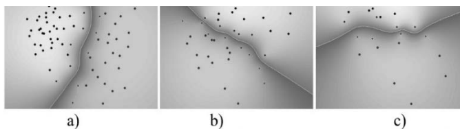
Fig.1. The results of SVM classification using different exponential cores: a) malicious traffic / non-malicious traffic; b) malicious traffic / spoofing traffic; c) malicious traffic / smurf traffic. (8пт, напівжирний)
